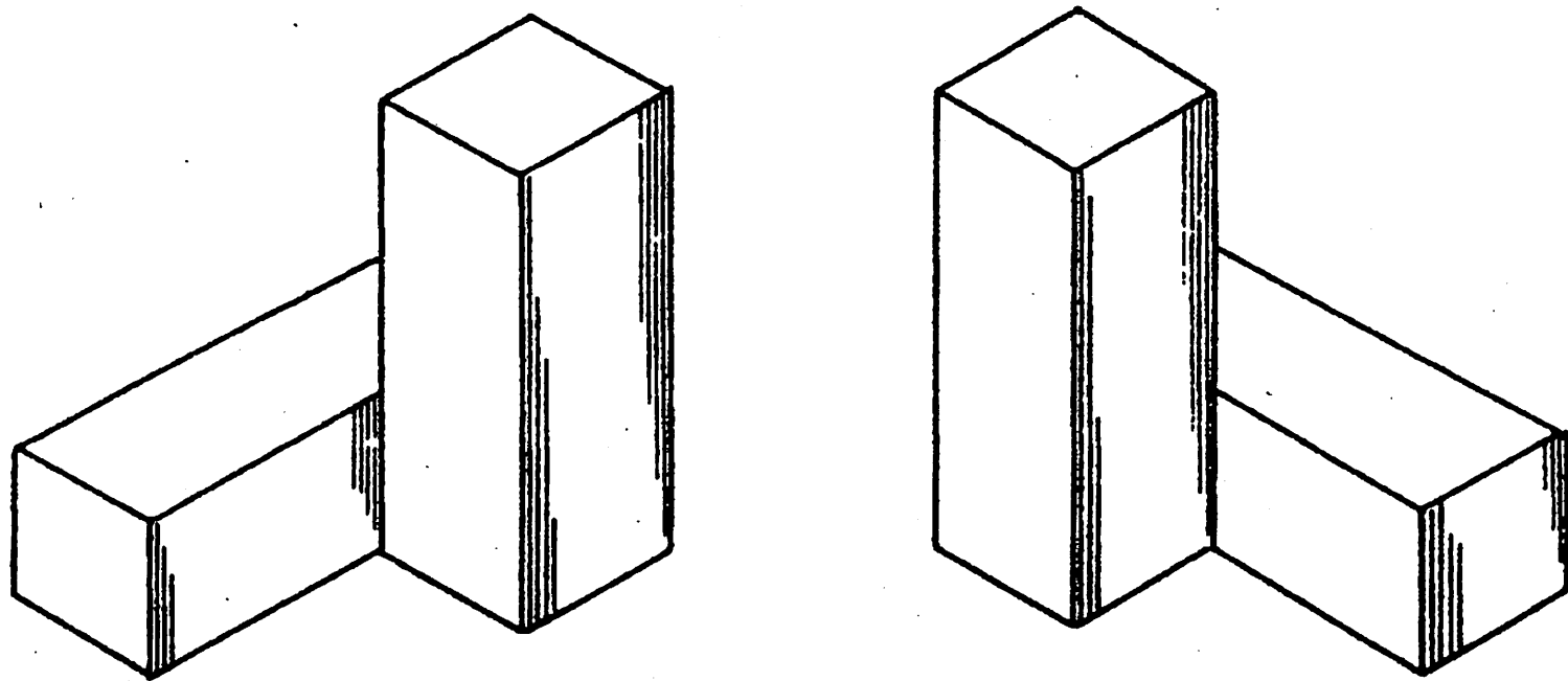
Figure 2 Enantiomorphous polyhedrons
